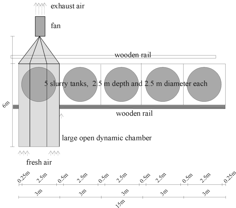
Figure 1. Design of the experimental facility for quantifying emissions from slurry stores (Amon et al. 2002).
